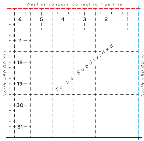
Figure 3-5. Regular order of completing exteriors where the south boundary was previously surveyed.
