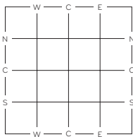
Figure 4-8. Key for marks on closing subdivision-of-section corners.
