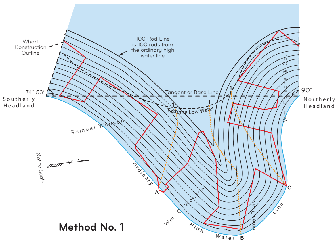
Figure 8-146. Method 1 for the division of tidewater flats.
