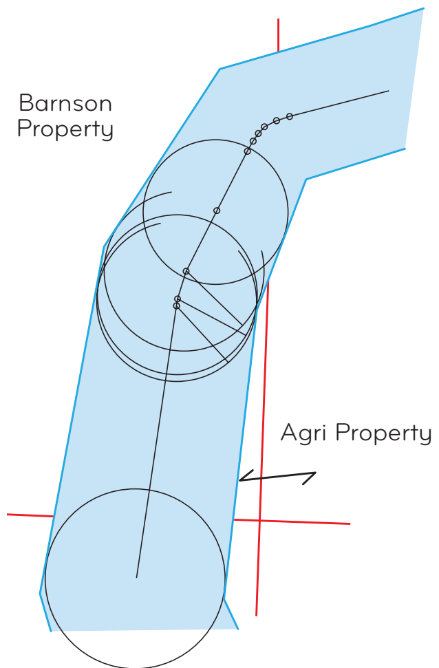
Figure 8-11. The medial line continues on the straight reach in this fashion to the end of the abandoned channel.
