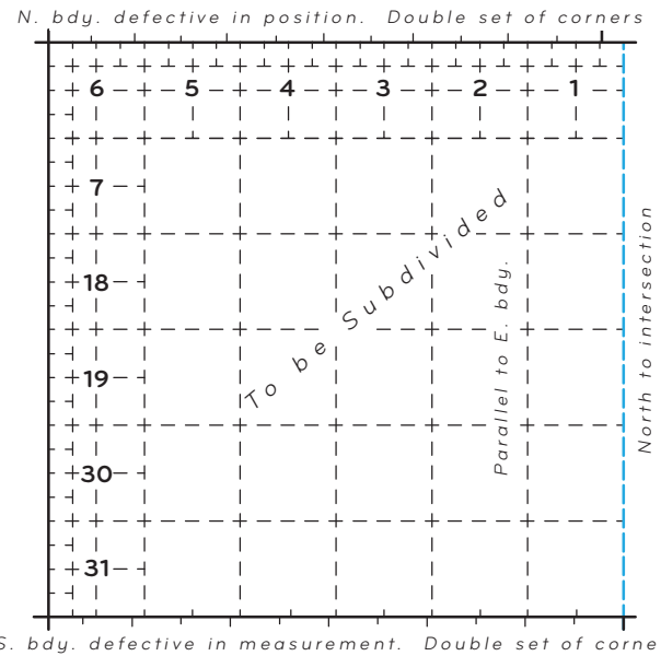
Figure 3-23. Rectification of a south boundary defective in measurement where the south, north, and west boundaries are fixed in position.
