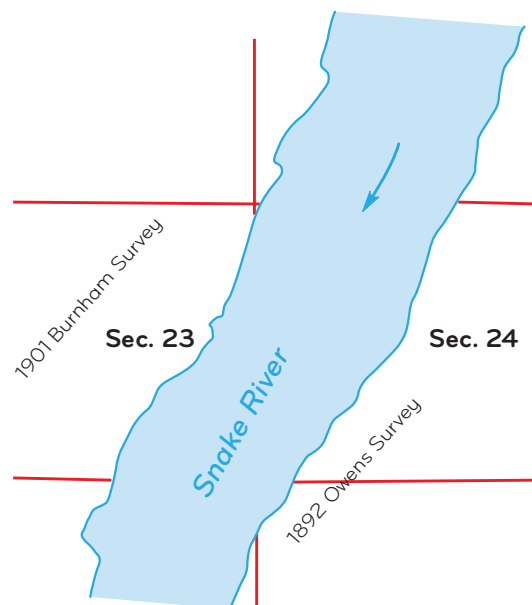
Figure 8-123. The Snake River was shown on the original GLO plats as about one-half mile wide although trees were growing in the river bed area at the time of the survey, according to tree-ring dating.
