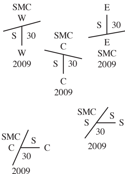
Figure 4-7. Key for marks on special meander corners.
