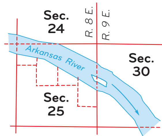
Figure 8-96. The disputed island from the original survey plats.
