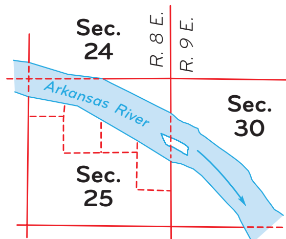
Figure 8-90. The disputed island from the original survey plats.
