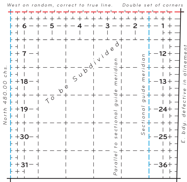
Figure 3-18. Rectification of a fixed east boundary defective in alignment.
