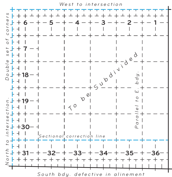
Figure 3-16. Rectification of a fixed south boundary defective in alinement.
