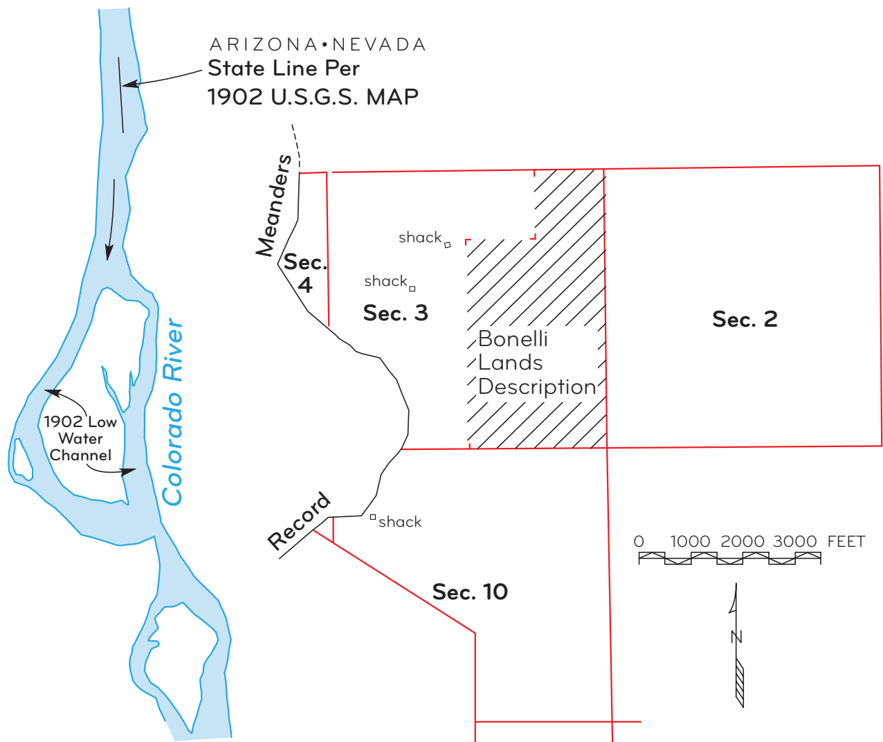
Figure 8-67. The Bonelli lands were over a mile from the Colorado River at the time of the 1905 original survey by the GLO. The river shown here is taken from a 1902 USGS survey map.
