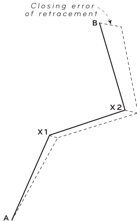
Figure 7-9. Adjustment of angle points on a meander line.
