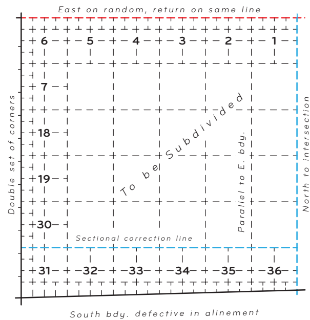
Figure 3-20. Rectification of a south boundary defective in alignment where both the south and west boundaries are fixed in position.
