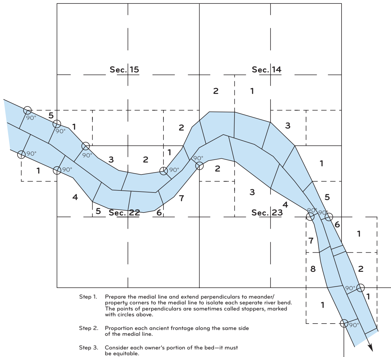
Figure 8-39. A method of apportioning the bed of a meandered nonnavigable river. Points were selected above and below the bend from which perpendiculars to the meander lines were extended to the medial line. The intervals along the medial line were determined by proportionate measurement.
