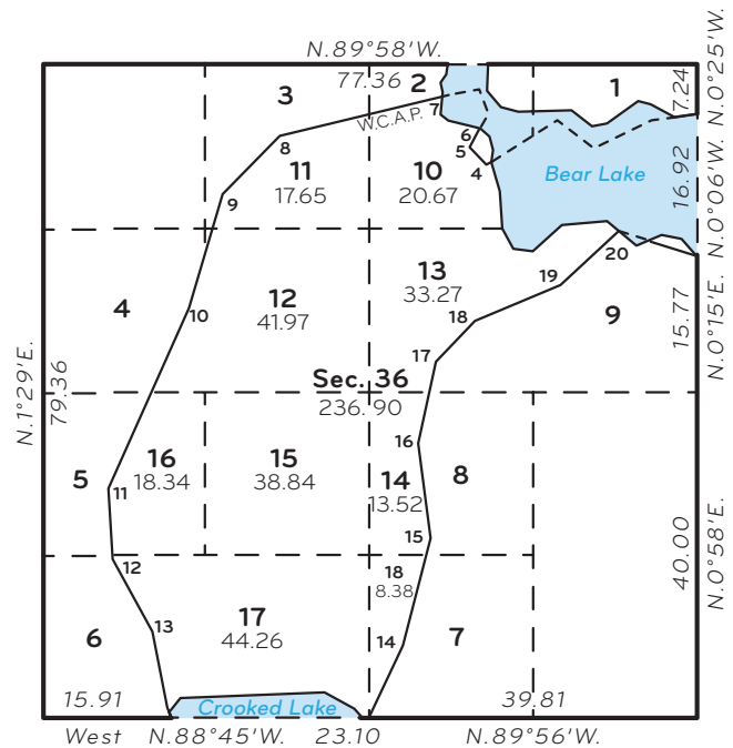
Figure 8-118. The Crooked Lake and Bear Lake case.
